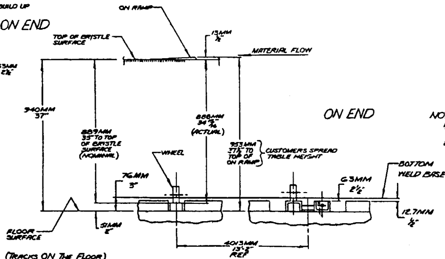
CONDITION #2 (TRACKS ON THE FLOOR) BUILT UP RECESS INSTALLATION OF FLOOR TRACKS FOR CONVENIENCE
